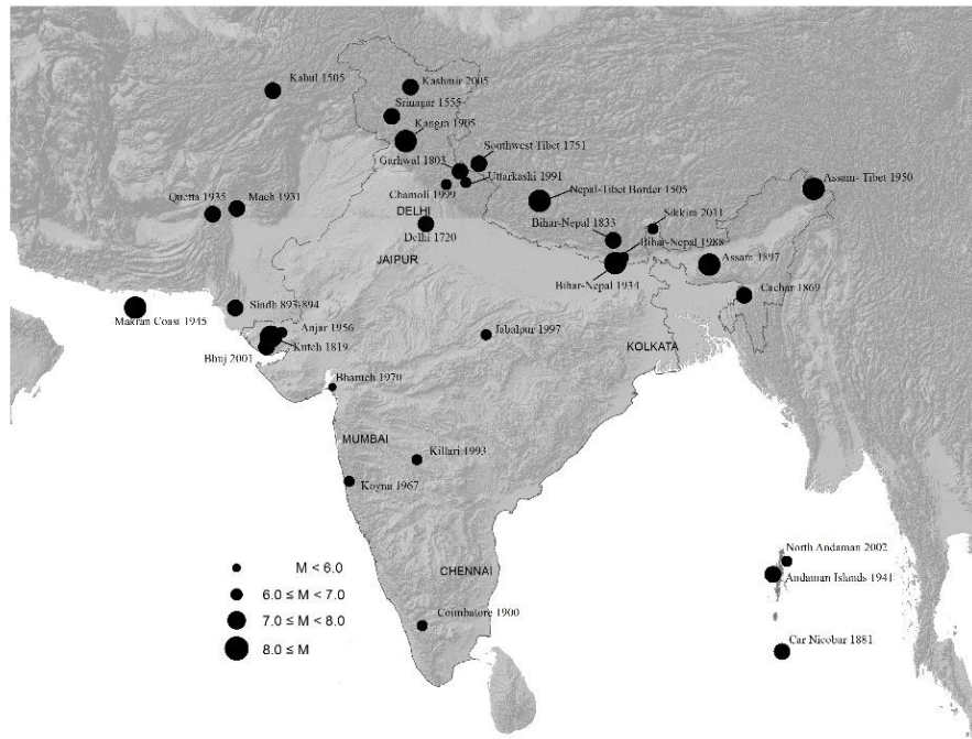
Figure 1. Prominent earthquakes in the Indian subcontinent (adopted from Jain (2016) under the terms of Creative Commons Attribution 4.0 International License available at http://creativecommons.org/licenses/by/4.0 ).
