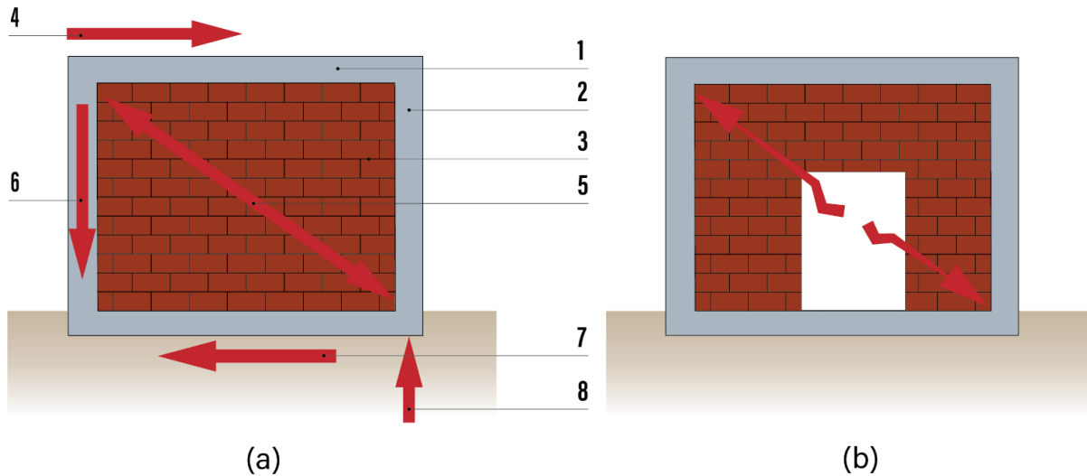
Figure 2. A strong confined masonry wall with tie beams (1), columns (2) and masonry (3). When an earthquake strikes (4) it is resisted by diagonal compression in the wall (5) and tension in a tie column (6). The horizontal earthquake force is resisted by the ground (7) and the vertical force also by the ground (8). In (b) the wall has an opening that prevents the formation of diagonal lines of force and that greatly weakens the wall.
