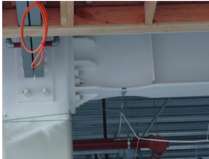
Figure 1. A building under construction with a column to the left and a steel beam connected to it. Note how the bottom plate (flange) of the beam near the column has been reduced in size. This area of deliberate weakening will be where a structural fuse will form in large earthquake. The steel in this region will stretch but not break.
