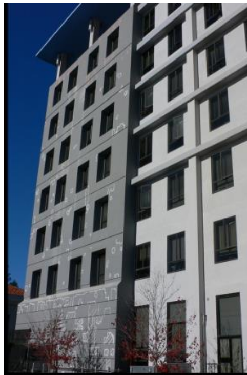
Figure 3. The thicker construction at the end of this building is a new concrete framework cast onto the existing structure for improved earthquake performance.
